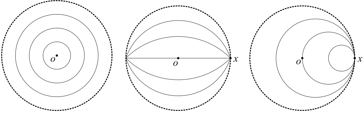
FIGURE 1. Orbit foliations of the actions of the groups K , A and N on \mathbb{RH}^2 , respectively.
